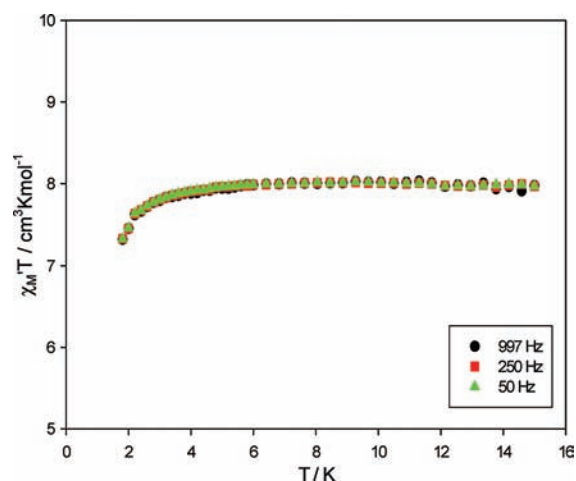
Figure 6. In-phase ( \chi'_M , plotted as \chi_M T vs T ) AC susceptibility of complex 1 \cdot 8\text{H}_2\text{O} \cdot 6\text{MeOH} in a 3.5 Oe field oscillating at the indicated frequencies.
