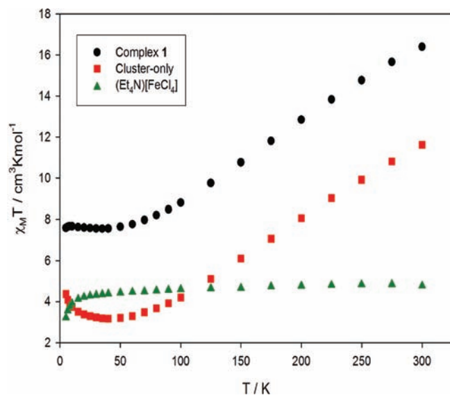
Figure 5. Plots of DC \chi_M T vs T for complex 1 \cdot 8\text{H}_2\text{O} \cdot 6\text{MeOH} and [\text{NEt}_4][\text{FeCl}_4] using data collected at 1.0 kOe. The difference plot, corresponding to the \chi_M T vs T for the \text{Fe}_7 cluster, is also shown.
