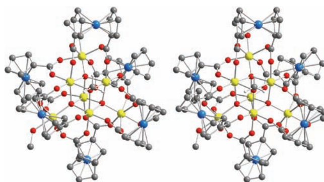
Figure 1. Pov-Ray stereopair of the structure of the [\text{Fe}_7\text{O}_3(\text{OMe})(\text{fdc})_6(\text{MeOH})_3]^{3+} cation of 1 . Hydrogen atoms have been omitted for clarity, except for those on the \mu_3 -methoxide ion.
