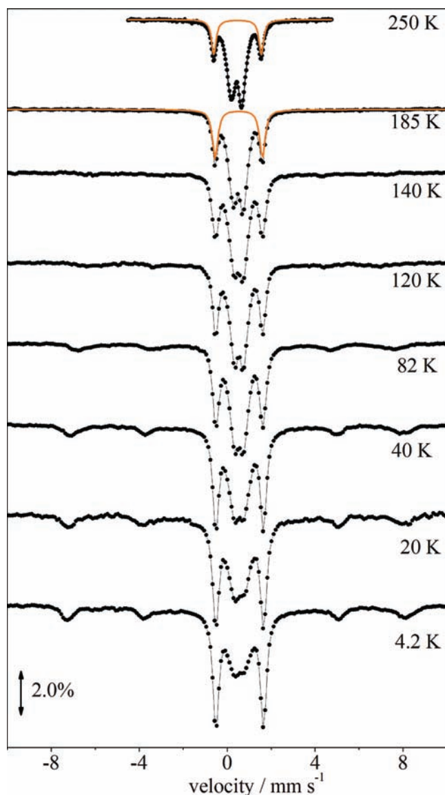
Figure 7. ^{57}\text{Fe} Mössbauer spectra in zero applied field for powder samples of 1 in the 4.2–250 K temperature range. The contribution of the ferrocene doublet is shown with the orange line.
